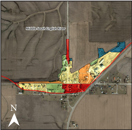
Figure 14. Modeled Nitrate Load in Webster, IA (lbs/acre/year). Source: UNI GeoTREE
