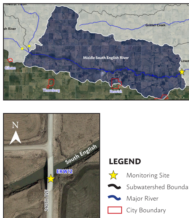
Figure 4. Water quality monitoring location for Middle South English River subwatershed. Source: ERW
