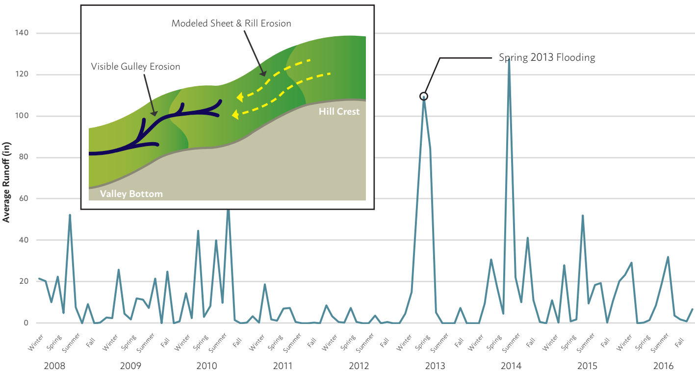
Figure 6. Average Runoff in Middle South English River (2008-2016). Source: DEP
