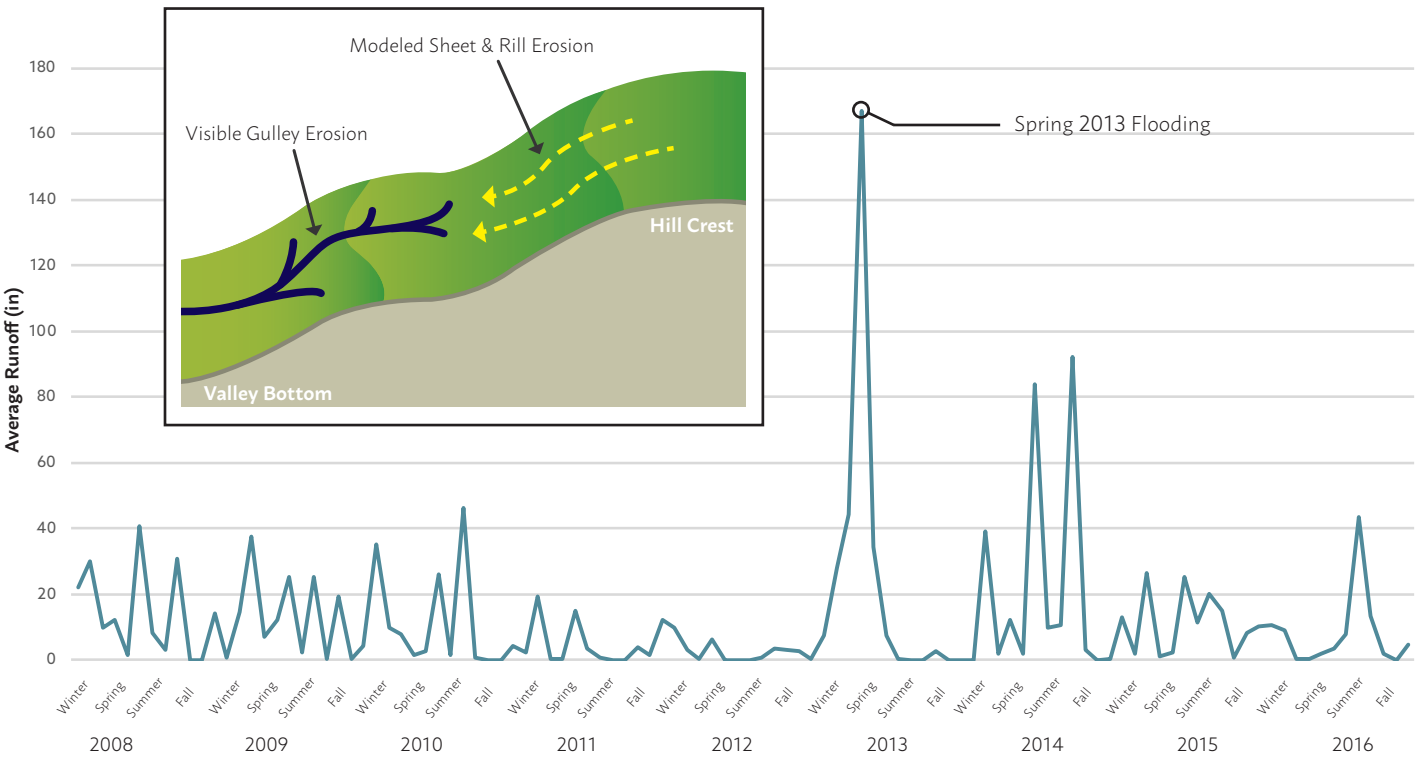
Figure 6. Average Runoff in the Lower North English River Subwatershed (2008-2016). Source: DEP
